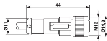
Dimensional drawing
